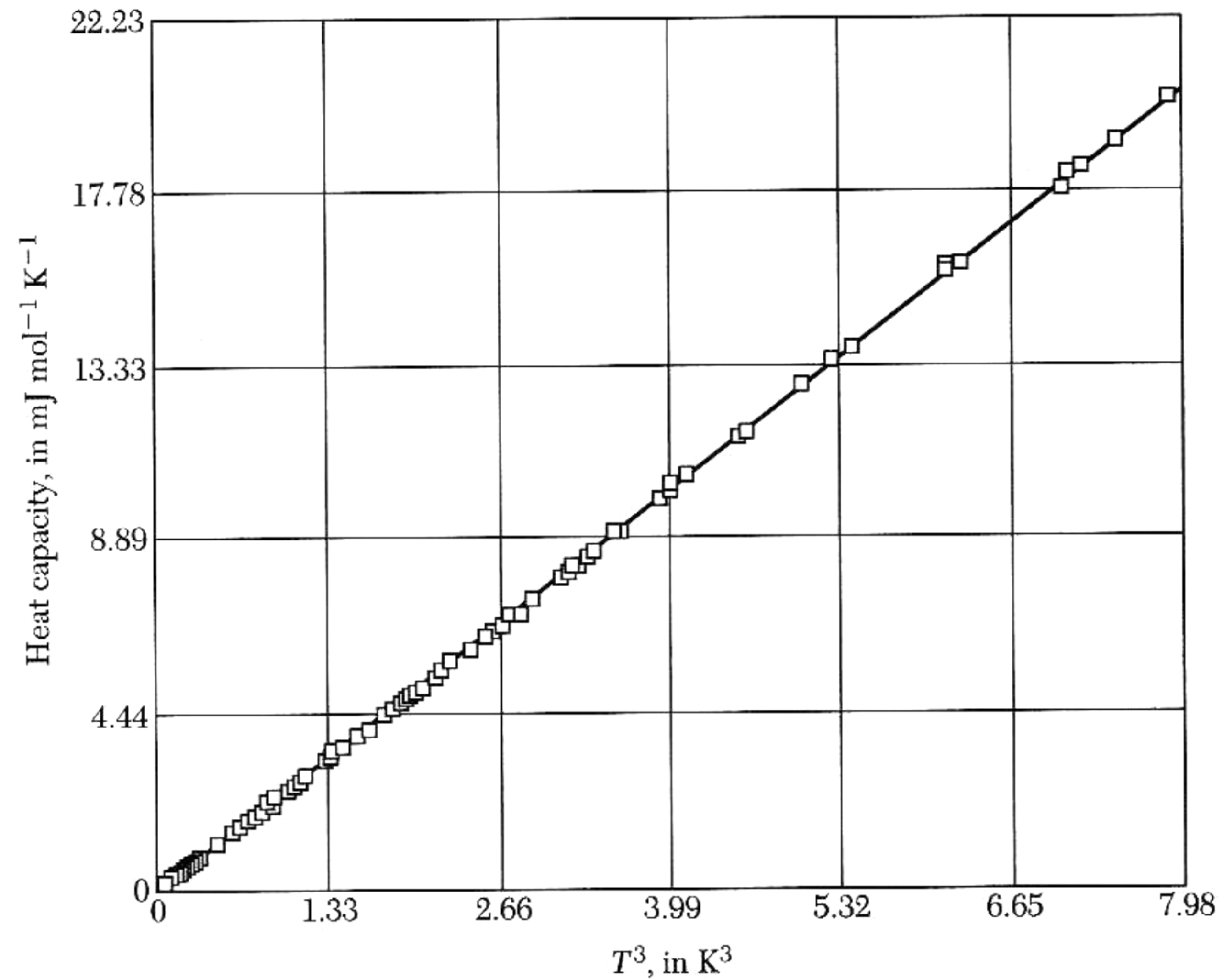
Heat capacity of Argon T = 0\text{K} to T = 2\text{K} (Kittel, Fig 9, Chap 5, 8th Edition)
